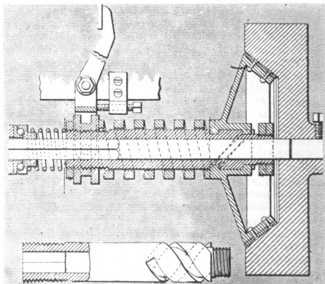
Section View of the Ireland Easy Release Clutch.
